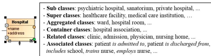
Fig. 1. Contextual information for a selected class [3].
